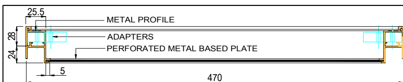
SECTION B-B
