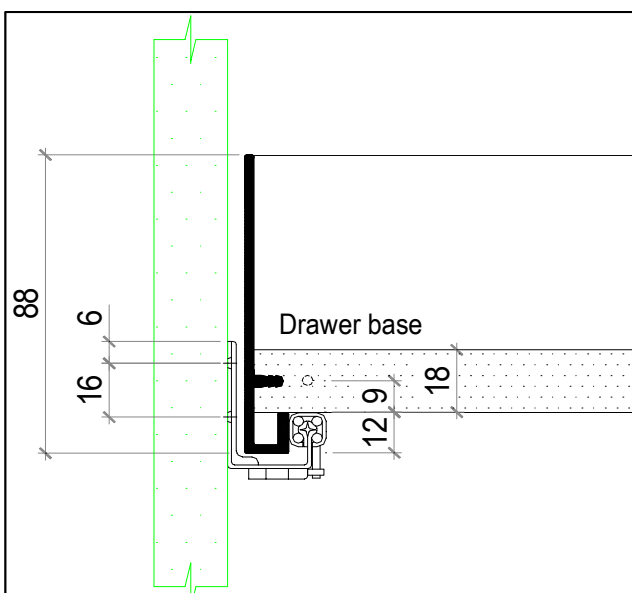
Drawer Side Details
