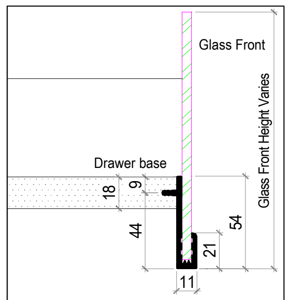
Drawer Front Details
