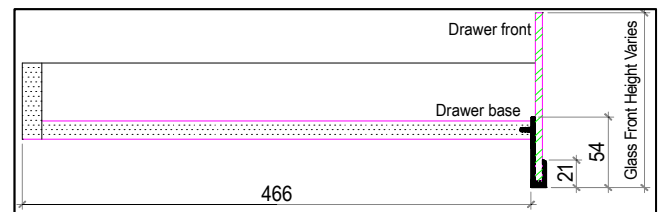
Drawer Side
