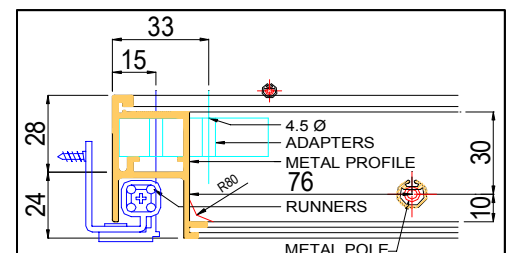
DETAILS 'A'
