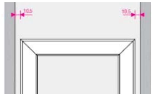
Width of tray = Carcass Internal - 21mm
